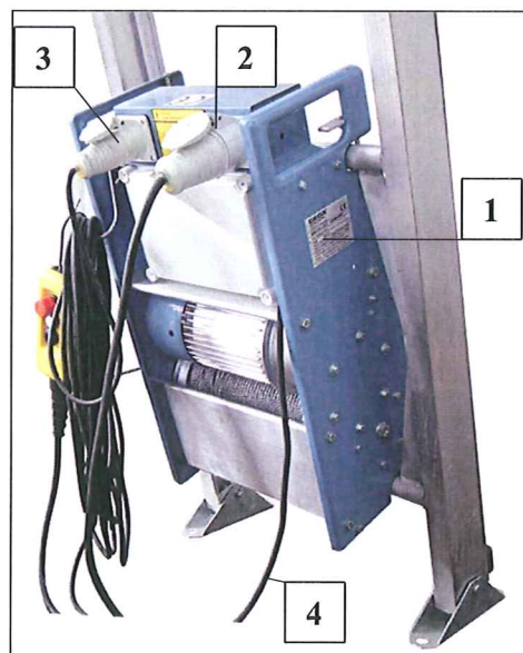
Fig. 6 Vinsch LIFT 250 COMFORT
